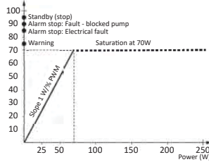
PWM feedback signal (power consumption)
